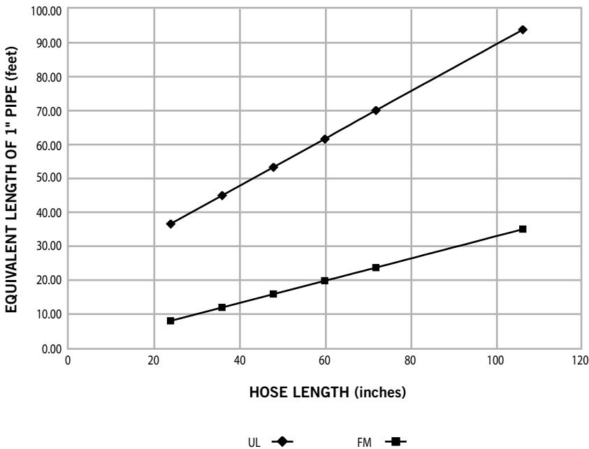
Friction Loss for 1/2"/12.7 mm Flexible Hose*
