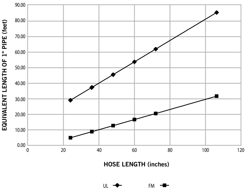
Friction Loss for 3/4"/14.47 mm Flexible Hose*
